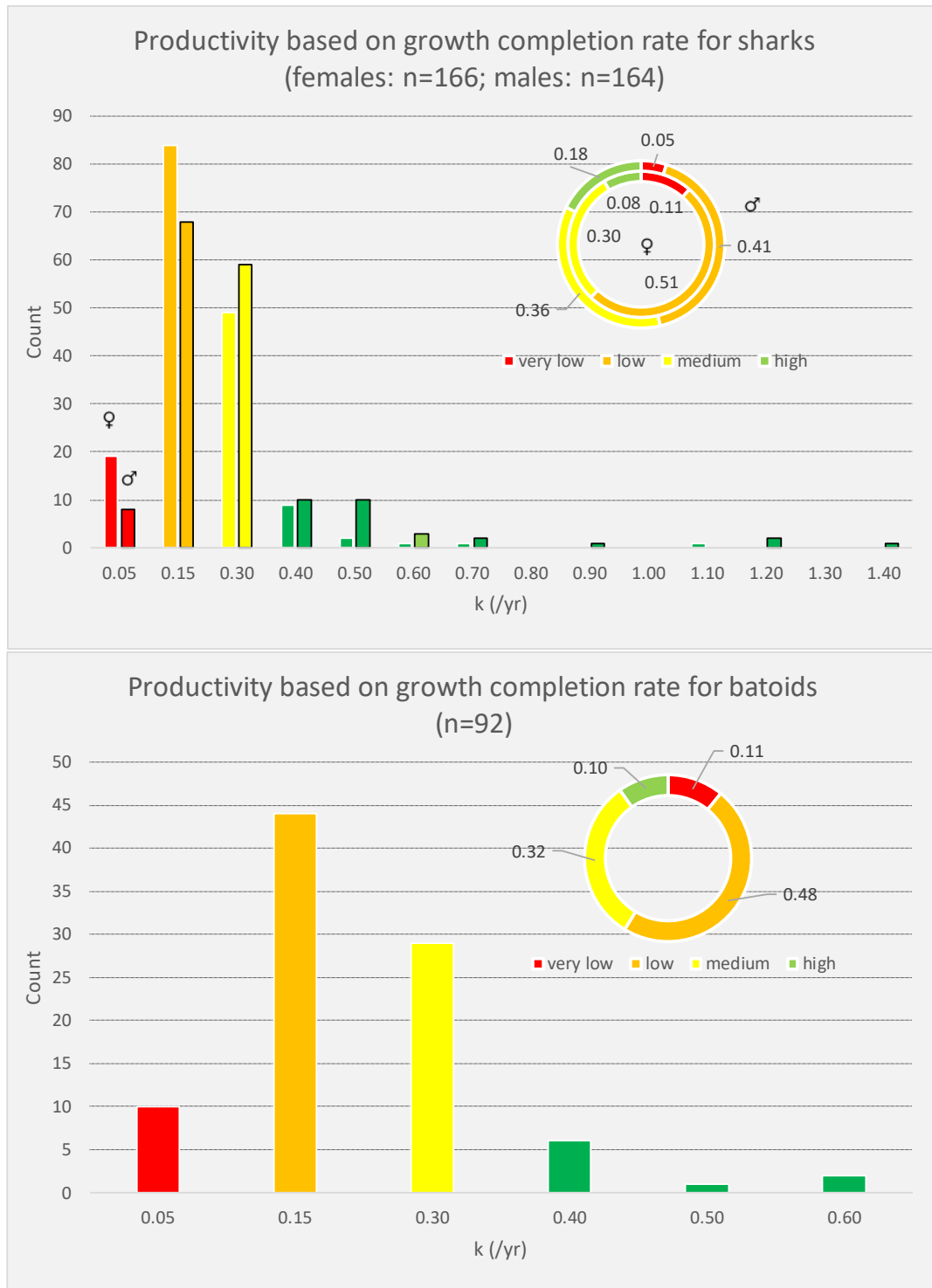
Figure 7. Classification of productivity into four categories (high, medium, low, and very low) according to the criteria for parameter k (growth completion rate from the von Bertalanffy growth curve) from Musick (1999). Top panel: sharks; bottom panel: batoids. For sharks, bars with black outline are for males and those without, for females. The inset pie charts show the percentage contribution of the species analyzed to each of the four productivity categories.
