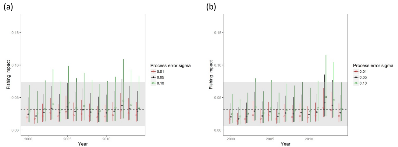
Figure I2: Annual impact (median values and 95% quantile range) estimated for (a) the Core Area and (b) the Assessment Area, using catchability estimates derived for three process error sigma values (0.01, 0.05 (base case scenario), and 0.10) (runs 2, 2e, and 2f - Table F1, Appendix F). Medium initial status (mean 0.5) and 100% capture mortality were assumed in each scenario. The dashed line is the mean value for the estimated r prior (0.03), with cv 0.6 (shaded grey area) (see section 4.4 for details).
