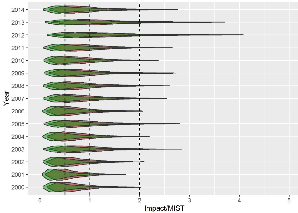
Figure 25: Annual sustainability risk for bigeye thresher in the Pacific, 2000-2014, as estimated for (a) the Core Area and (b) the Assessment Area. Sustainability risk and uncertainty are distinguished based on the occurrence (green) or absence (red) of post-capture survival. Sustainability risk (x-axis) is the ratio of total impact (combined values across three initial population status assumptions) to the maximum impact sustainable threshold (MIST) (here corresponding to the maximum intrinsic rate of population increase r ). A ratio above one indicates potentially unsustainable fishing impact.
