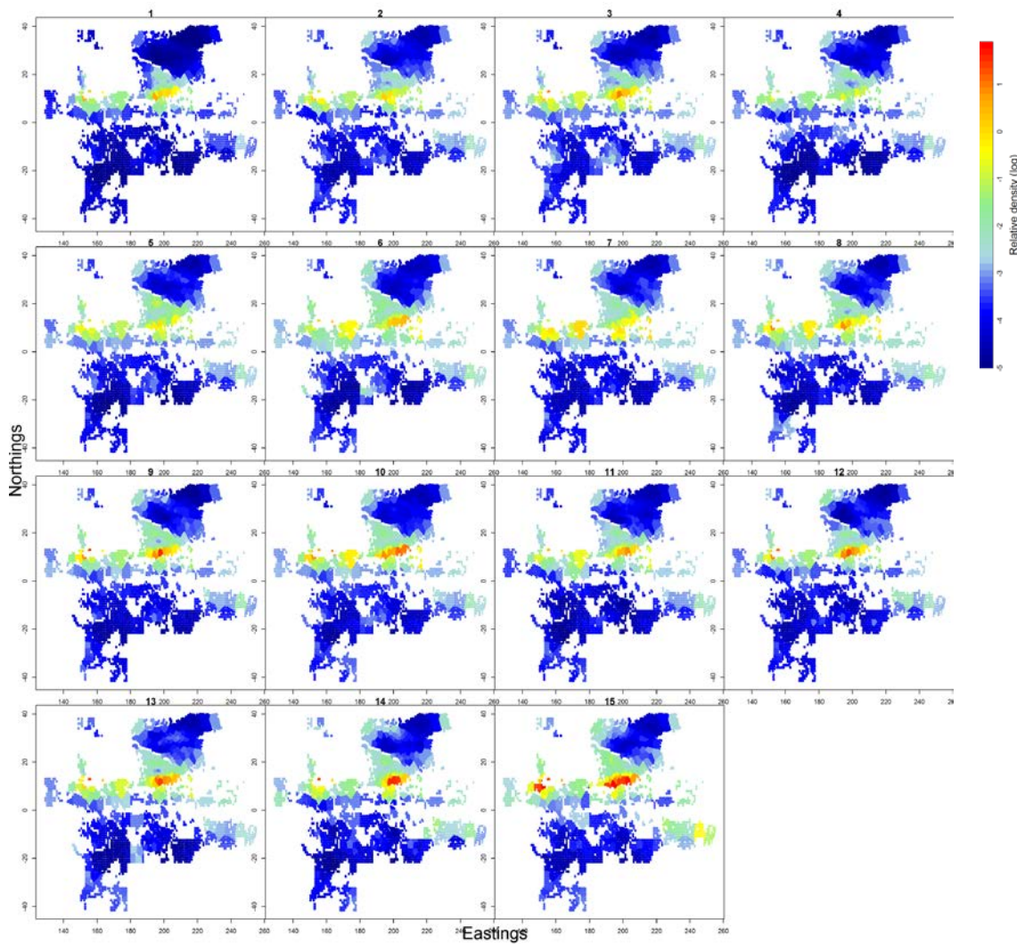
Figure 13: Fine-scale, annual relative density estimates (log scale) for bigeye thresher in the Assessment Area, from 2000 (top-left) to 2014 (bottom-right), as predicted from the spatial-temporal delta-GLMM model. Annual data are plotted in 10x10 km grid cells used to standardise and extrapolate catch rates in all GLMM models.
