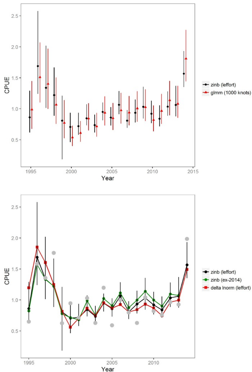
Figure 17: Annual CPUE indices of relative abundance (mean and 95% CI) for bigeye thresher in the Calibration Area, 1995-2014, predicted using (a) the final ZINB model and the delta-GLMM model fitted with 1000 knots; and b) the final ZINB model, the same ZINB model excluding year 2014, and a delta lognormal GLM model. All models were fitted to US Hawaii observer data from the Calibration Area. Grey dots in (b) are nominal (unstandardised) CPUE. All indices were normalised to the mean of each series to allow comparison.
