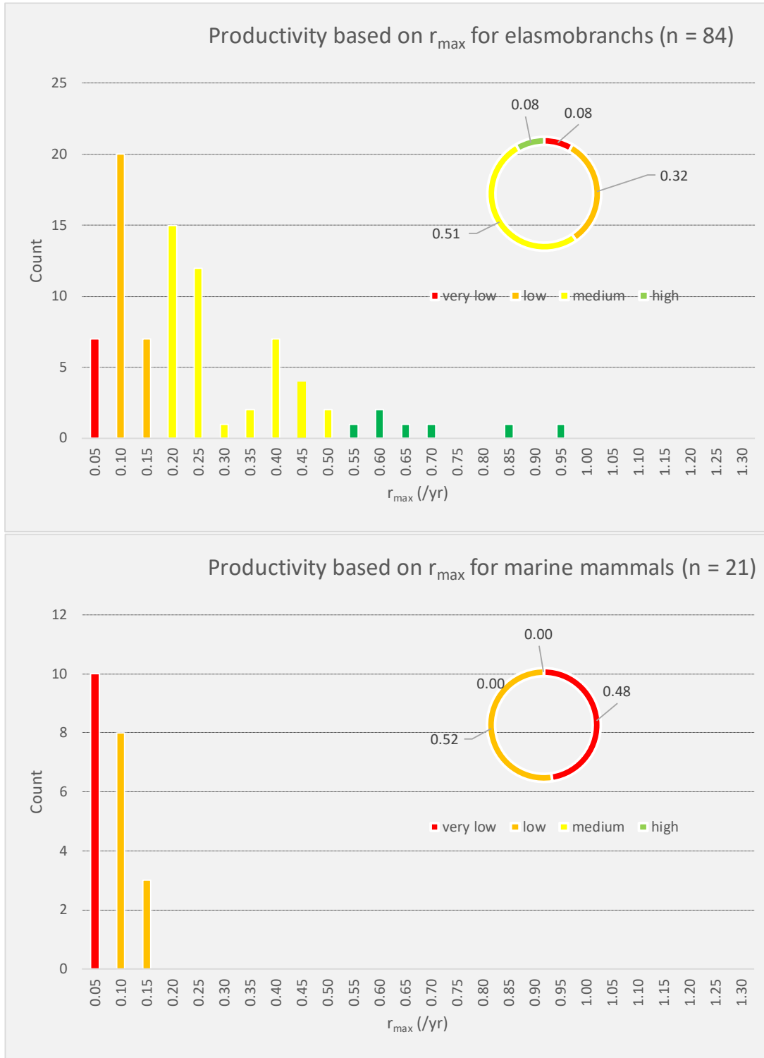
Figure 17. Classification of productivity into four categories (high, medium, low, and very low) according to the criteria for r_{max} from Musick (1999). Top panel: elasmobranchs; bottom panel: marine mammals (all data from Finucci et al. (2024)). The inset pie charts show the percentage contribution of the species analyzed to each of the four productivity categories.
