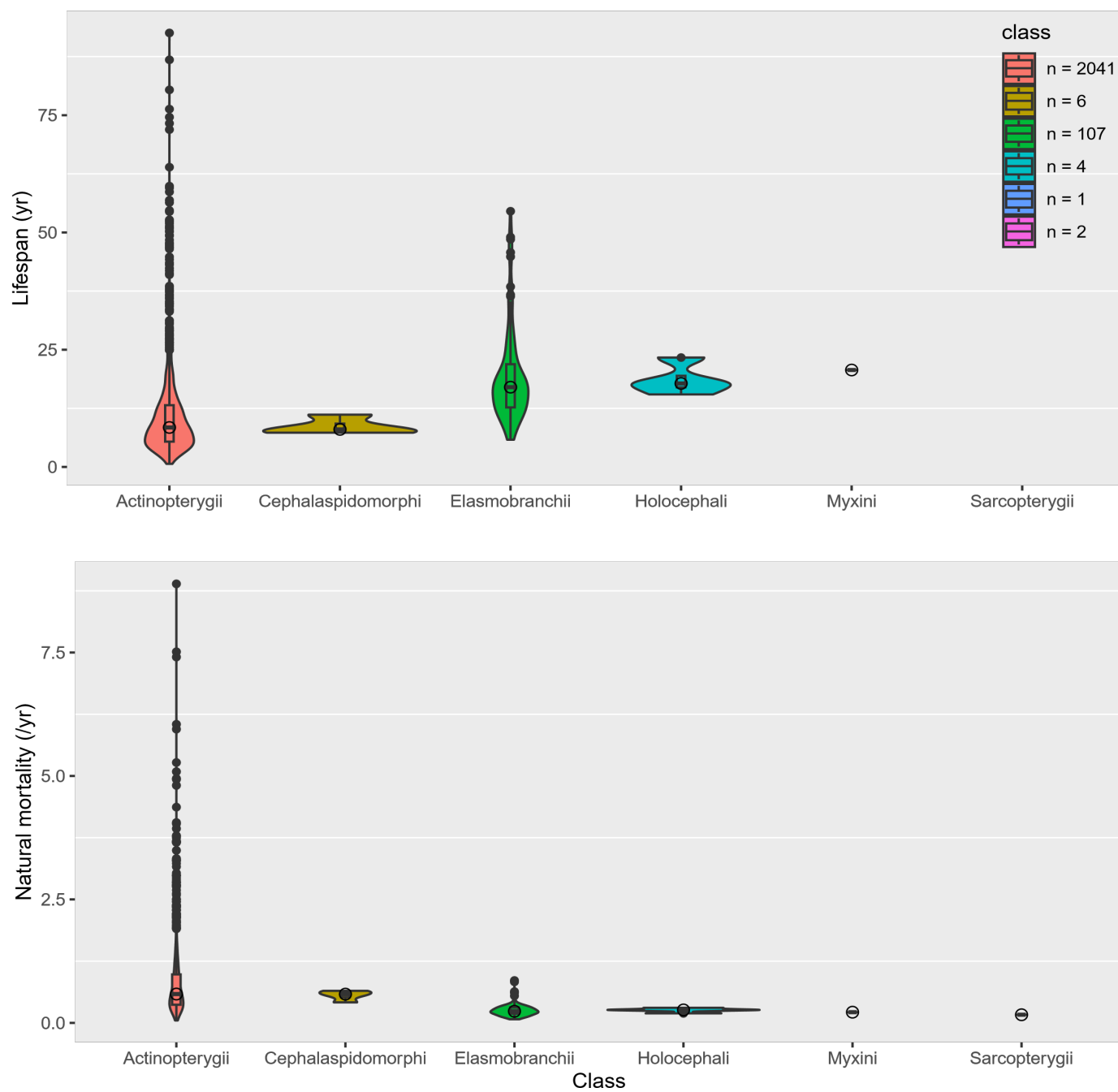
Figure 13. Violin/box plots of the distribution of lifespan (top) and natural mortality (bottom) for classes of fishes included in data from Thorson et al. (2023) extracted from FishBase. The violin plot indicates density of points; inside the violin are the median (dash), mean (circle), interquartile range (25th to 75th percentile; box), 1.5 x IQR (whiskers), and outliers (dots).
