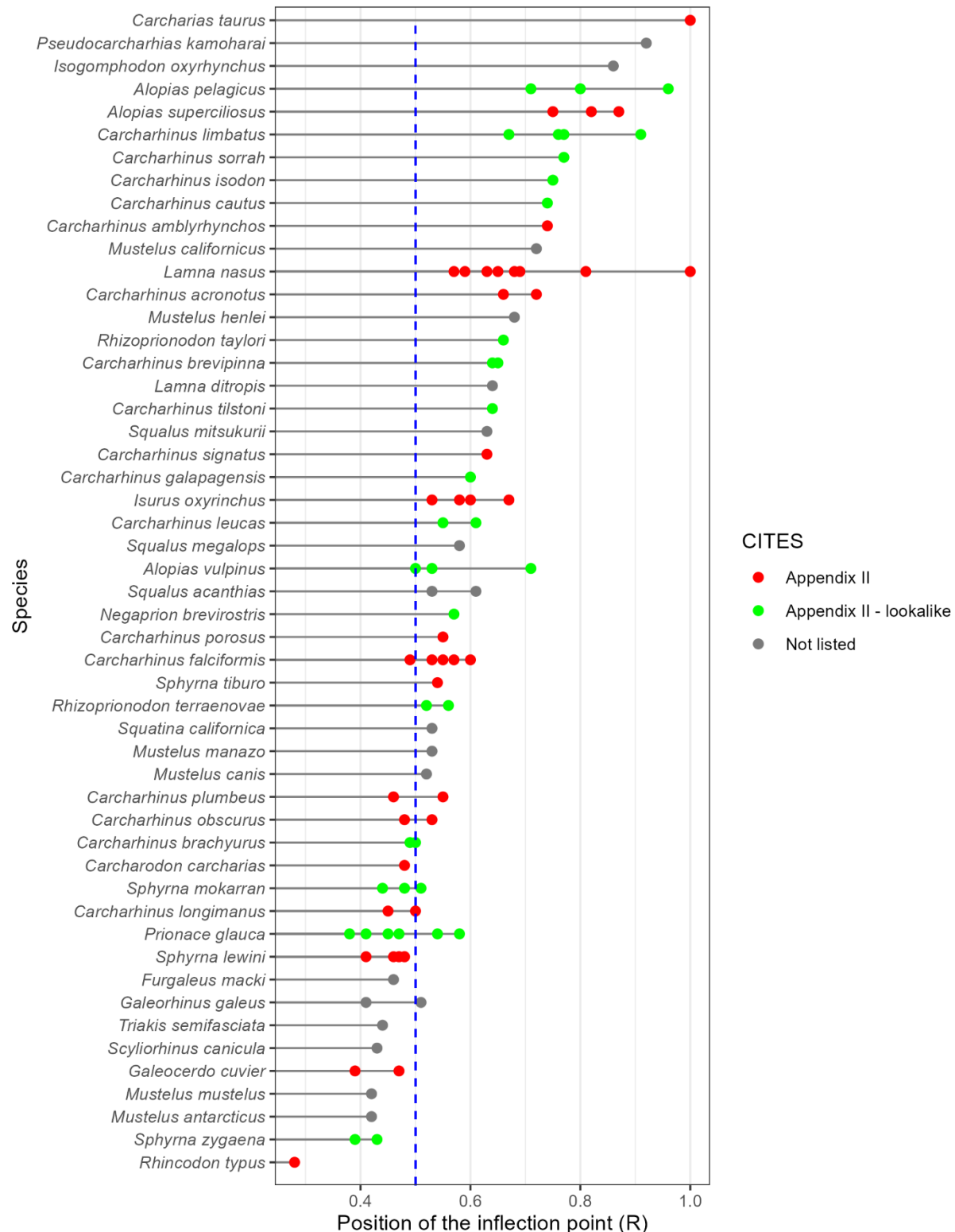
Figure 25. Position of the inflection point of population growth curves (R) for sharks (data from Cortés (2016) augmented, n = 101 ) according to CITES listing and “lookalike” status. The vertical blue dashed line indicates when the MSY (maximum sustainable yield) is reached at half the carrying capacity (0.5K). All species with R values to the left of this line would have a higher capacity to withstand population declines. More than one point for a given species indicates multiple populations or studies.
